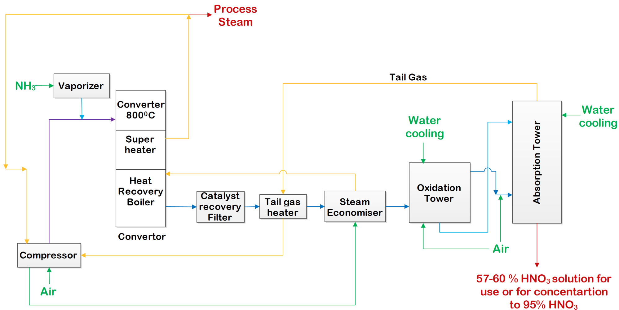
Figure: Manufacturing of Nitric acid by oxidation of ammonia
